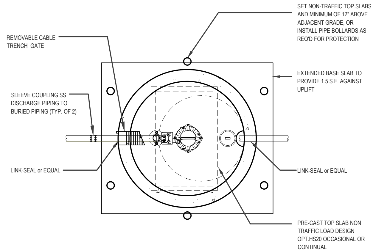
PLAN VIEW MUNI 104 WET WELL
