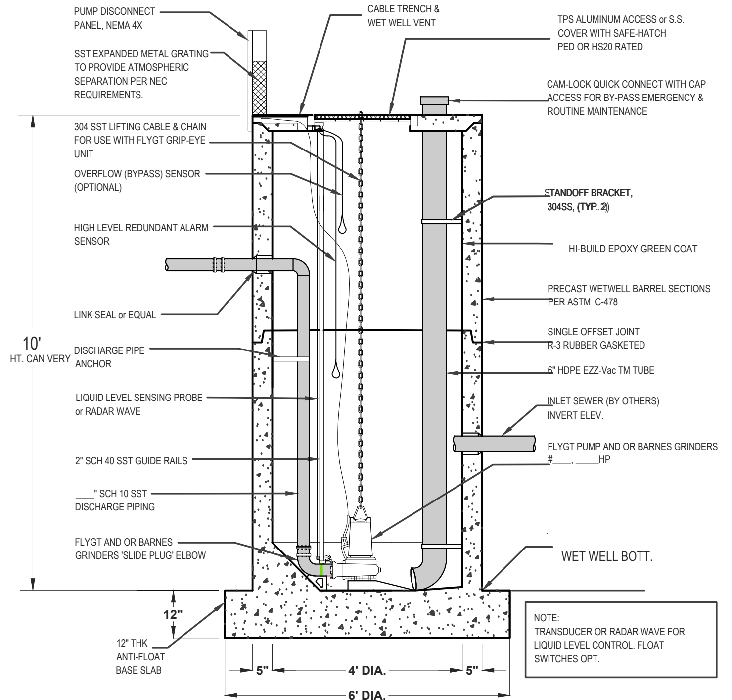
SECTION VIEW MUNI 104 SIMPLEX SS LIFT STATION
